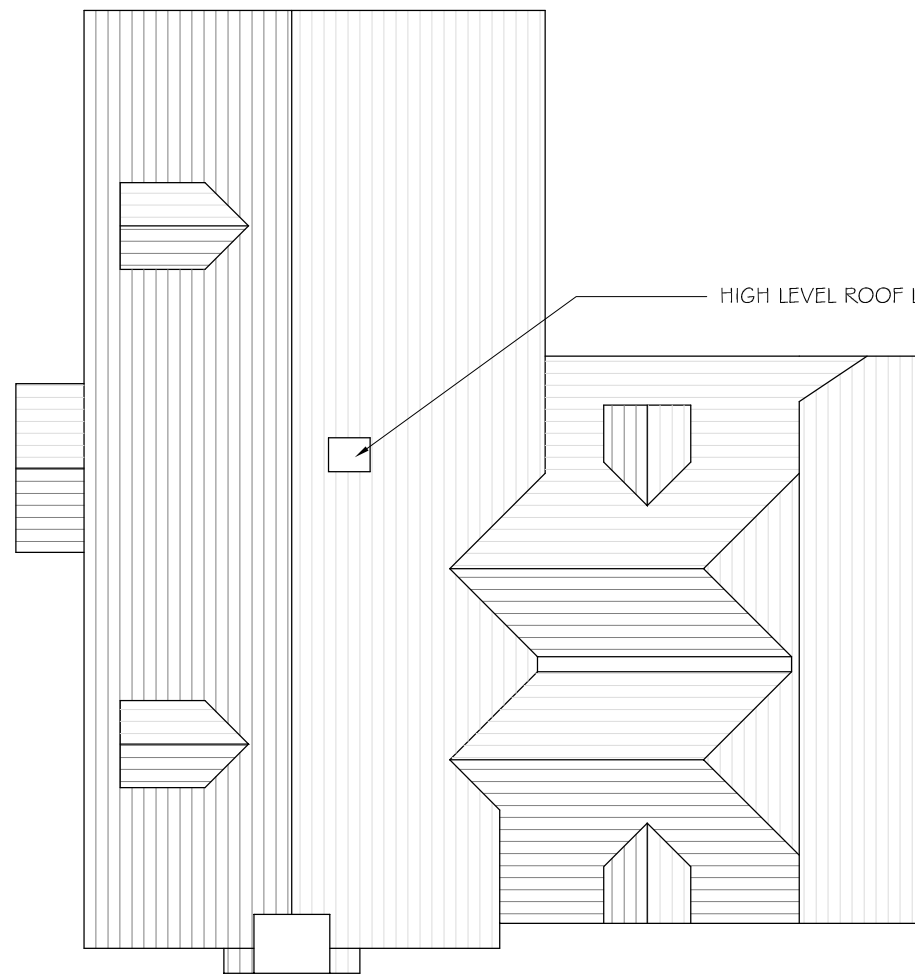
ROOF PLAN 1:100
