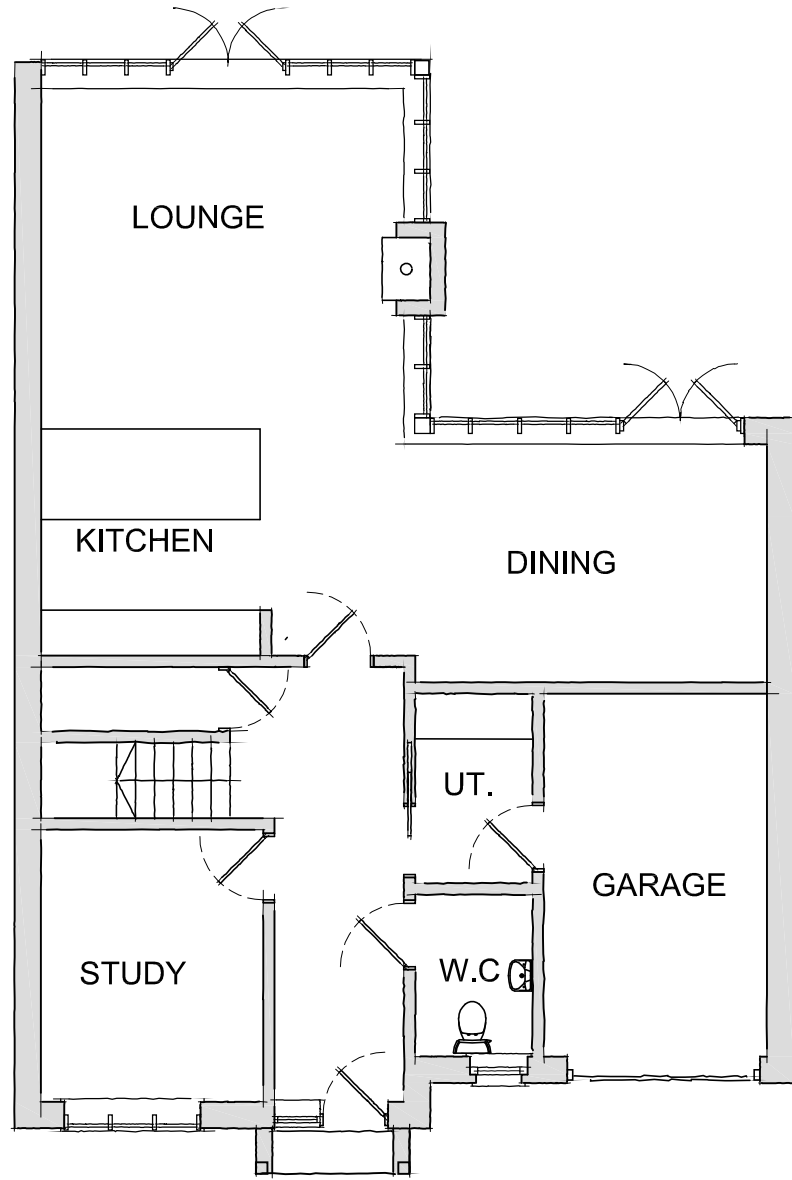
GROUND FLOOR 1:100
